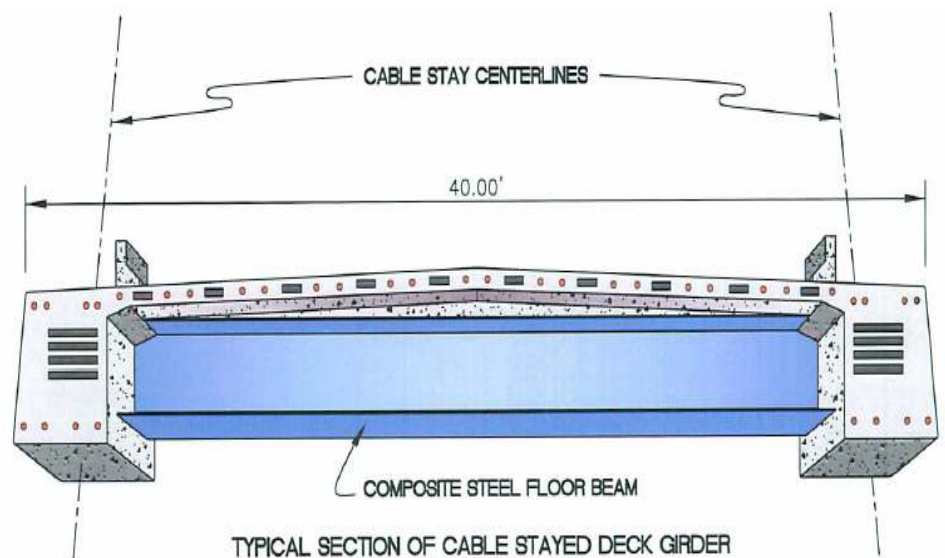
FIGURE 3: Diagram of the composite, steel, deck slab beam
