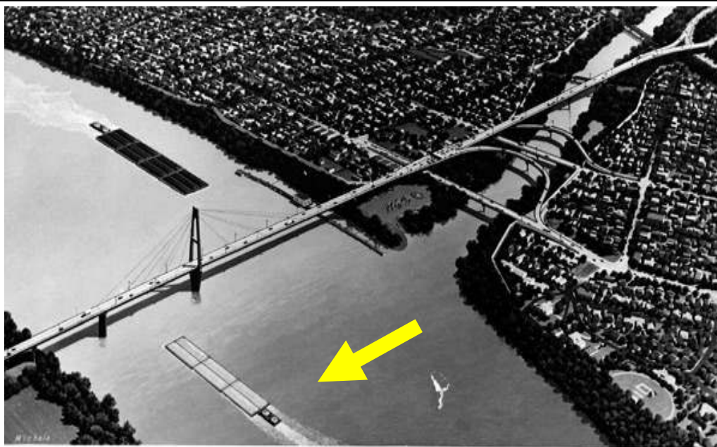
FIGURE 1: Southeast view of original, mid-stream, pylon location for the East Huntington, steel, cable-stayed bridge
