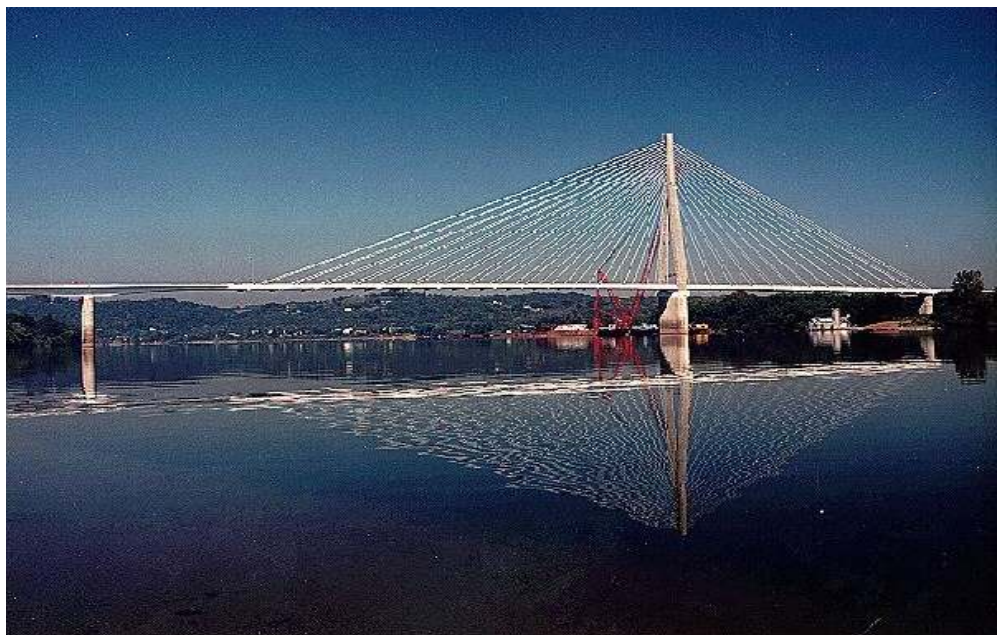
FIGURE 5: The Ohio River reflects east elevation of hybrid , main span girder; pier 2 cantilever (L), cable-stayed (R).
